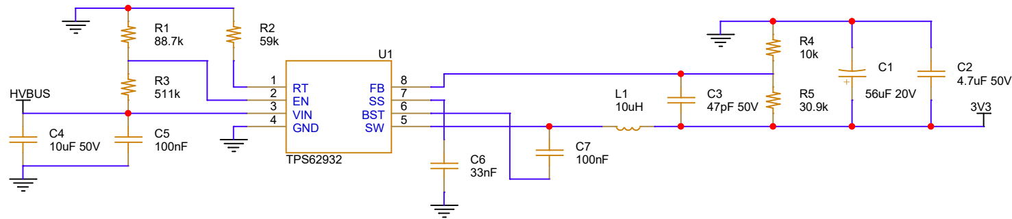
8-30V UNREG BUS TO 3V3 2A 371MHz SWITCHING DC/DC
