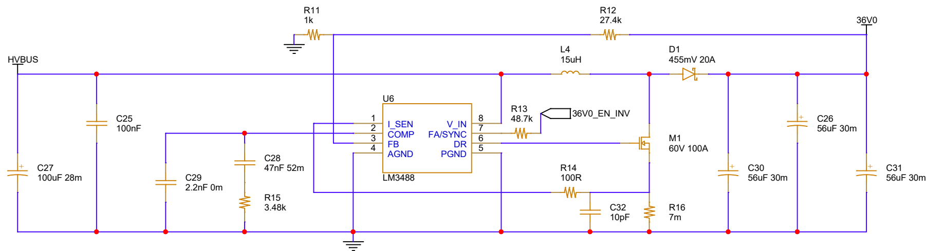
15-30V UNREG BUS TO 36V0 3A 336MHz SWITCHING DC/DC
