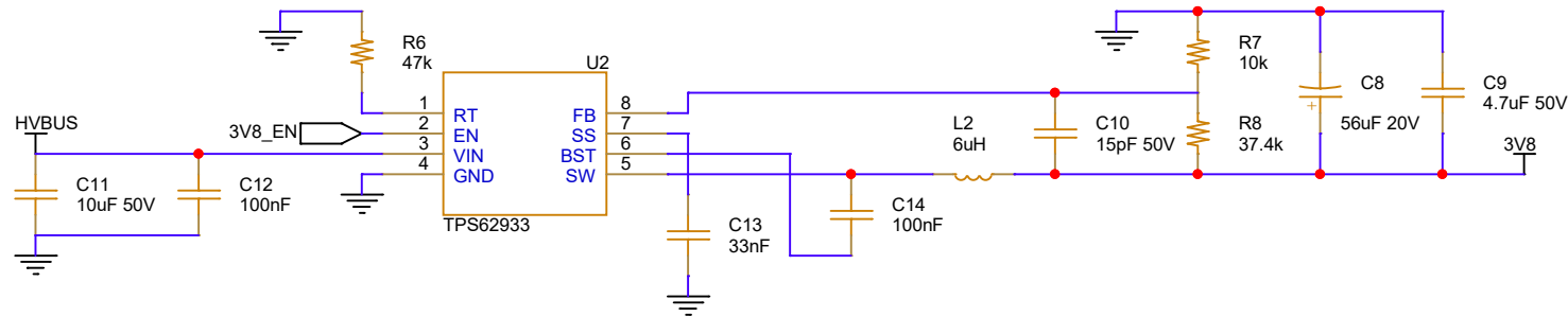
8-30V UNREG BUS TO 3V8 3A 460MHz SWITCHING DC/DC
